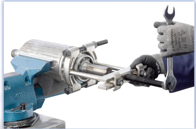
Back puller extraction
