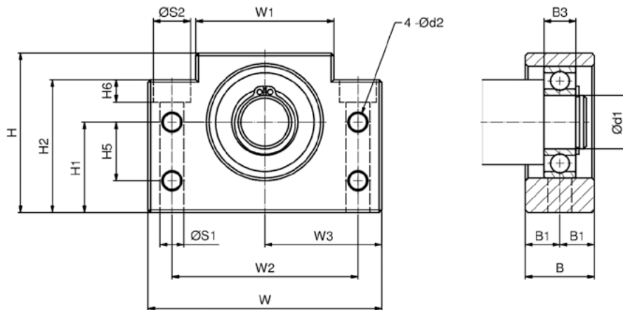
Figure 6.17 __ Dimension floating bearing unit BF and EF
