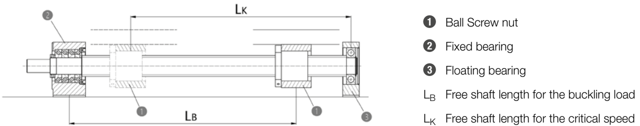
Figure 2.21 __ Bearing arrangement fixed - supported
