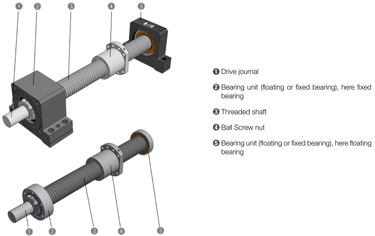
Figure 1.1 ___ Construction of a Ball Screw drive
